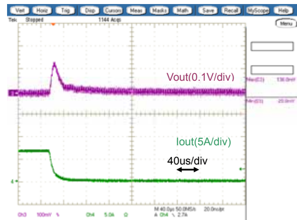
Fig.7-2-8. Load Transient Response ( I_o=6A 0A)
